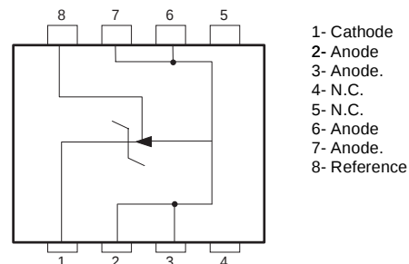
SO8 (Top view)
